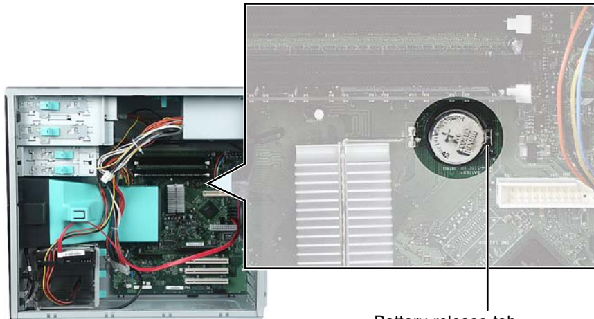
Battery release tab
